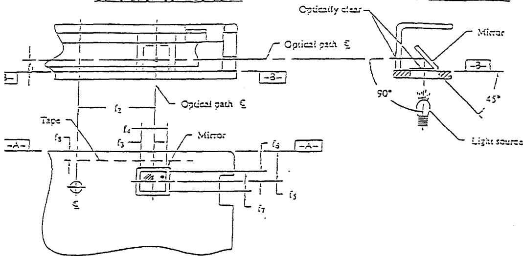
Test configuration
