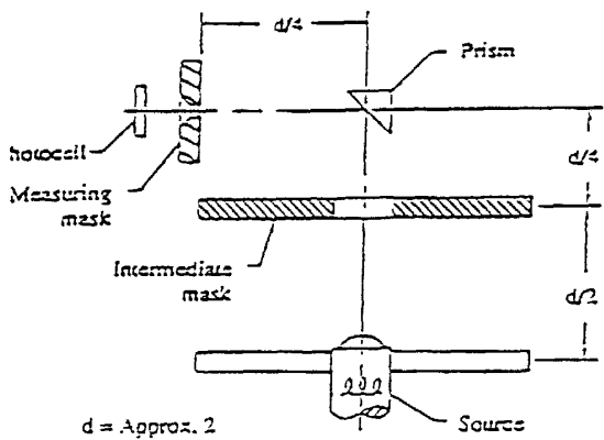
Calibration configuration
