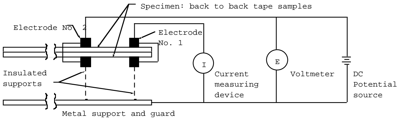
Figure 4 - Tape resistance measurement circuit
