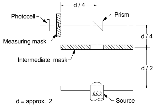
Calibration configuration
