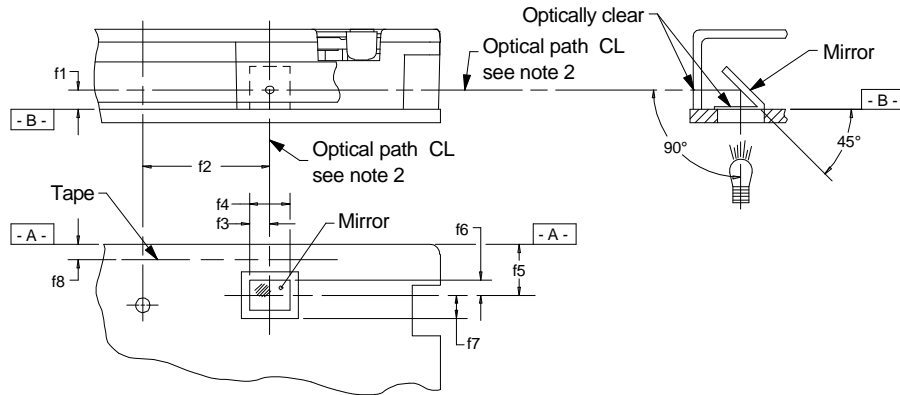
Calibration configuration
