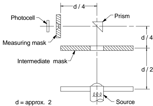
Calibration configuration
