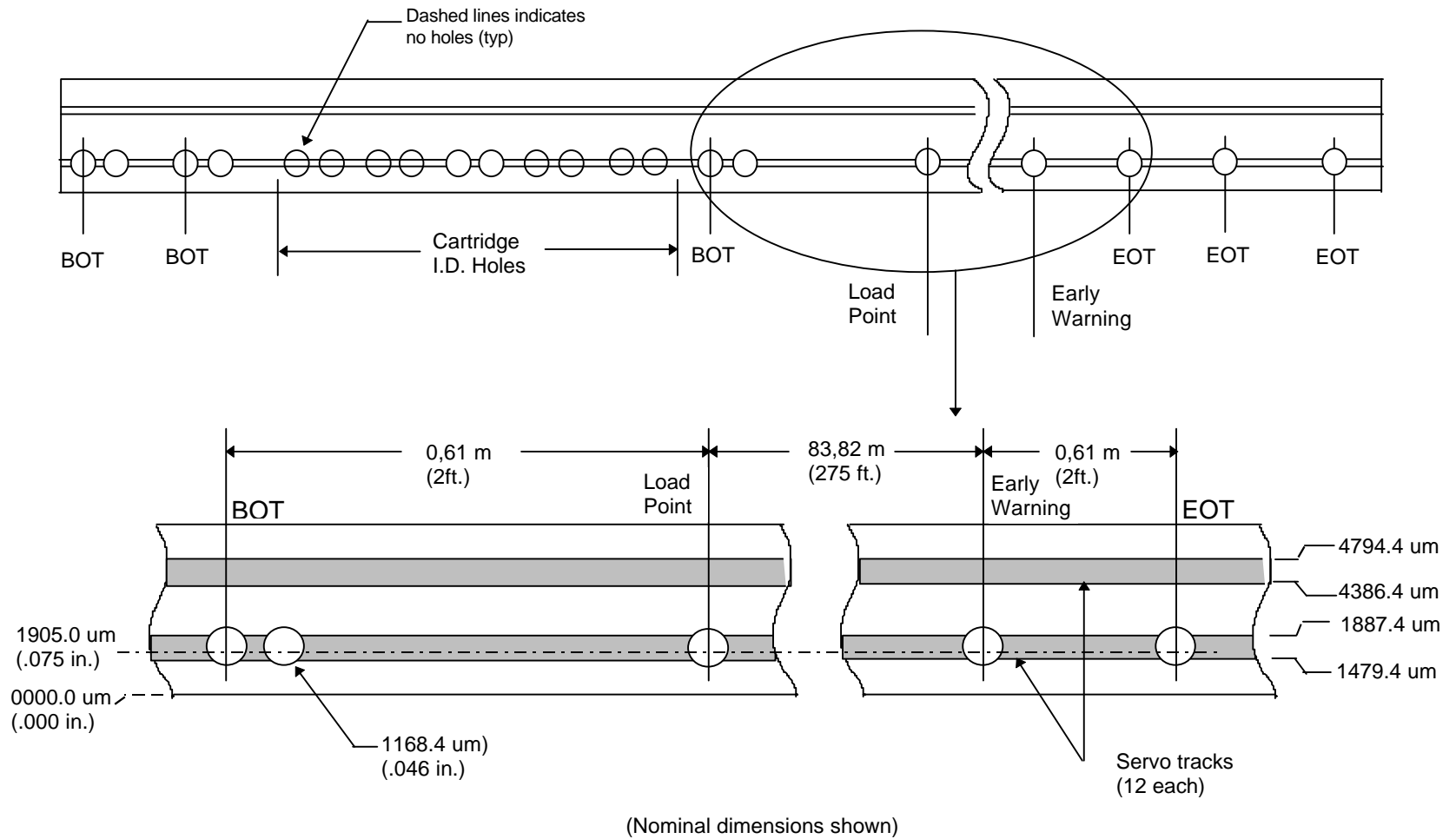
Figure A.3 Servo track / hole relationship Track pitch: 34um Center guard hard: 51 um
