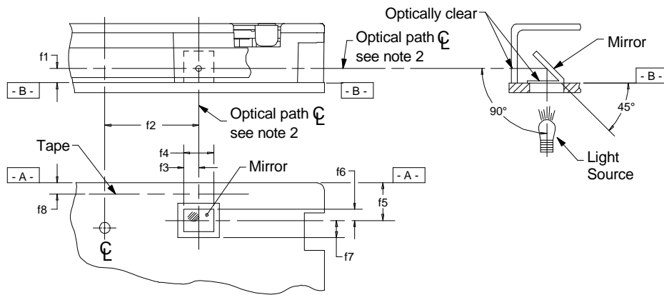
Calibration configuration
